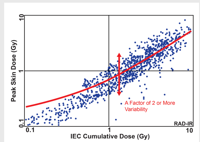
Figure 3: Cumulative air kerma (referred to here as “IEC Cumulative Dose”) shows an improved correlation with peak skin dose, as illustrated in the above plot adapted from the RAD-IR study 10 . However, a variability of more than a factor of two is still observed between the cumulative air kerma and peak skin dose.
