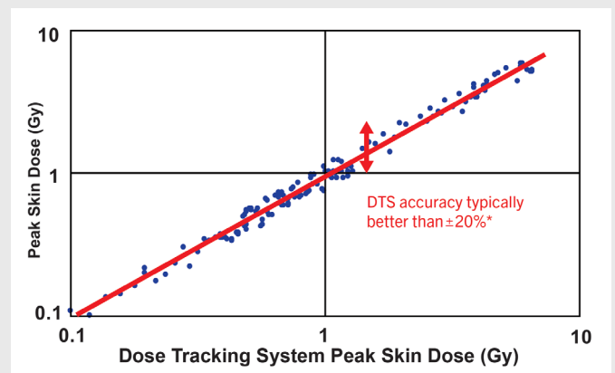
Figure 5: Illustrative plot demonstrating typical accuracies of the estimation of peak skin dose provided by the DTS to within \pm 20\% , with appropriate patient graphic selection and positioning. Presently, no alternatively reliable methodology exists.
